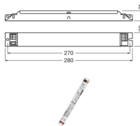
Specificaties Osram LED Driver OPTOTRONIC 55/220-240/1A0 CS L G2
